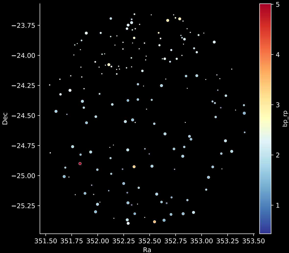
APOGEE DR17 Field: [K2_C2_357+13_btx] Stars: 177
