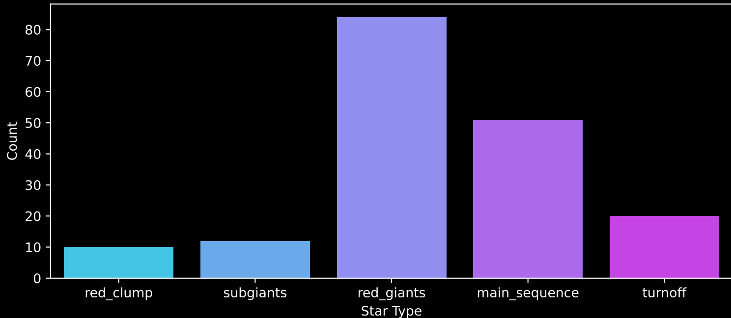
APOGEE DR17 Field: [K2_C2_357+13_btx] Count plot of Star Type
