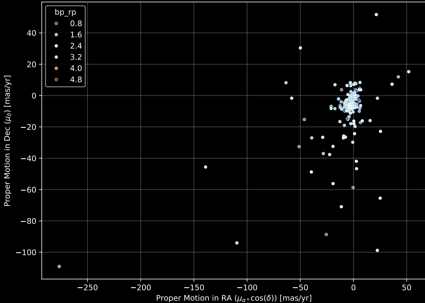
APOGEE DR17 Field: [K2_C2_357+13_btx] Proper Motion Diagram (n= 177)
